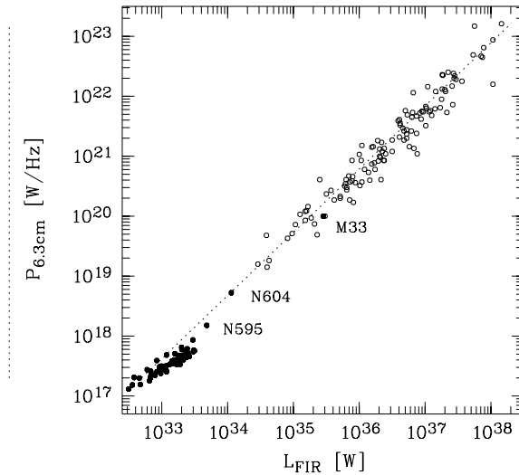
Figure 10. Plot of the monochromatic radio luminosity versus the FIR luminosities for M 33 (Hippelein et al. 2003) and its star-forming regions (filled circles) together with the data for the Effelsberg 100-m galaxy sample (Wunderlich et al. 1987, open circle). The dotted line has a slope of 1.10 (Wunderlich & Klein 1988).
