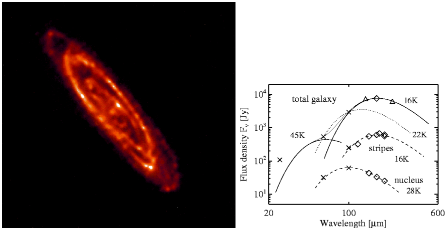
Figure 1. Left: ISOPHOT 170 \mu\text{m} map of M 31 (Haas et al. 1998), with an angular resolution of 1.3' . North is towards the top, and East is towards the left. The field size is 2.9 \times 2.9 degrees. Right: Infrared SED of M 31 (Haas et al. 1998). The data are shown by symbols (diamonds ISO, crosses IRAS, triangles DIRBE) with the size being larger than the errors. The blackbody curves with emissivity proportional to \lambda^{-2} are shown by lines. The dotted line with T=22 K through the IRAS 60 and 100 \mu\text{m} data points indicates what one would extrapolate from this wavelength range alone without any further assumptions.
