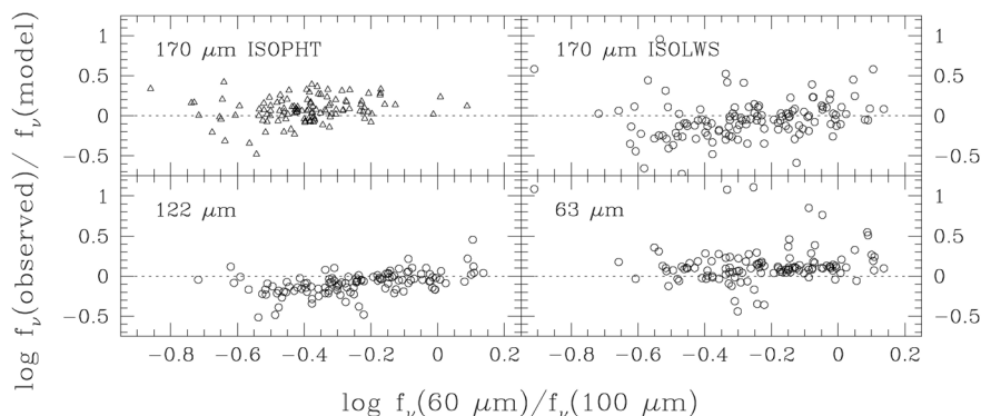
Figure 12. Comparison of observed FIR continuum levels observed by ISO with the model predictions of Dale & Helou (2002). The circles derive from the ISO LWS templates and the triangles represent 170 \mu\text{m} data from the ISOPHOT Serendipity Survey (Stickel et al. 2000).
